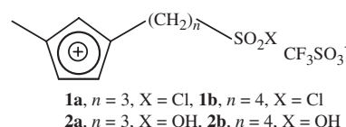
Scheme 1. Acidic ionic liquids.
